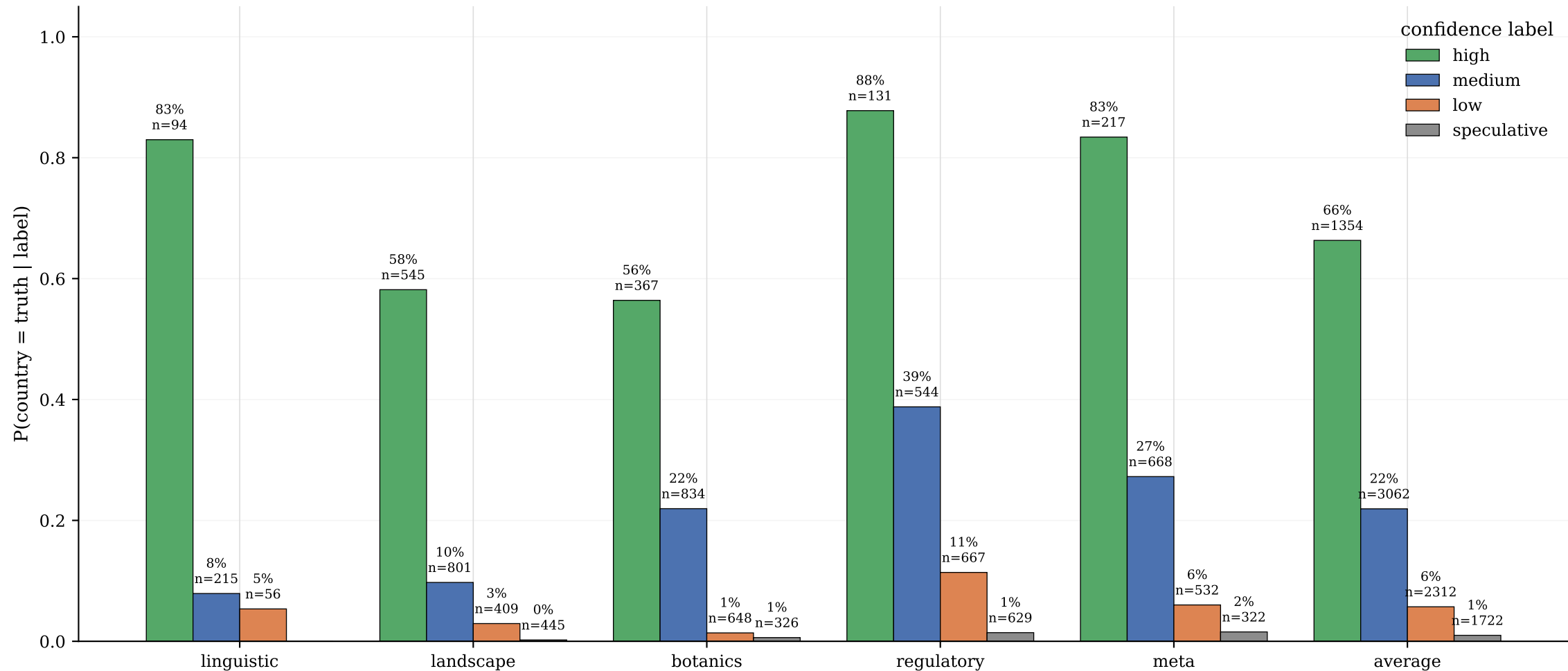
Per-label hit-rate, how often does a labeled candidate match the ground truth?
